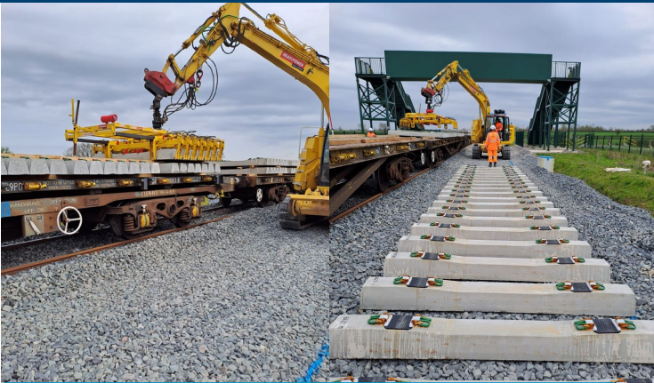
Sleeper installation in Twyford
